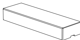
COPING 383 15 \times 47\frac{1}{4} \times 7" 383 x 1200 x 180mm
