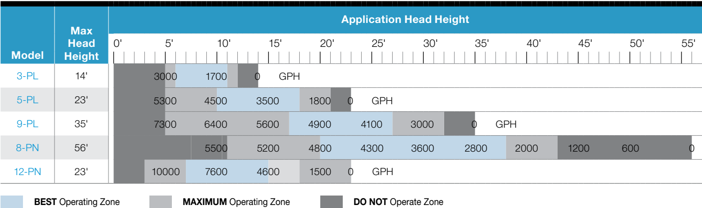
Aquascape PL & PN Series Pump Flow Chart (GPH)
